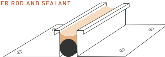
BACK-TO-BACK CASING WITH BACKER ROD AND SEALANT
